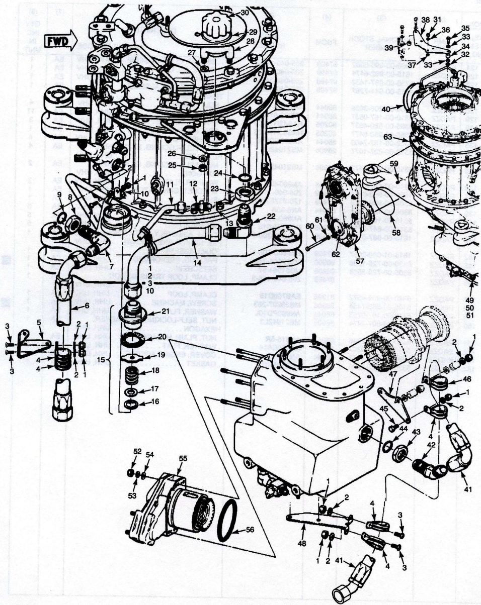
Figure 154. Transmission Assembly.
