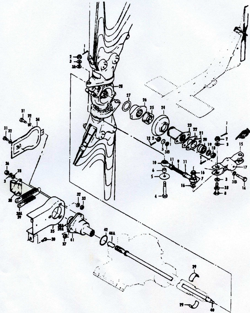
Figure 145. Tail Rotor Installation
