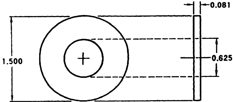
Figure D-364. Number: 5310-UH1-038-1, WASHER Fabricate from: NSN 9380-00-143-7110 Material: Rubber Sheet
