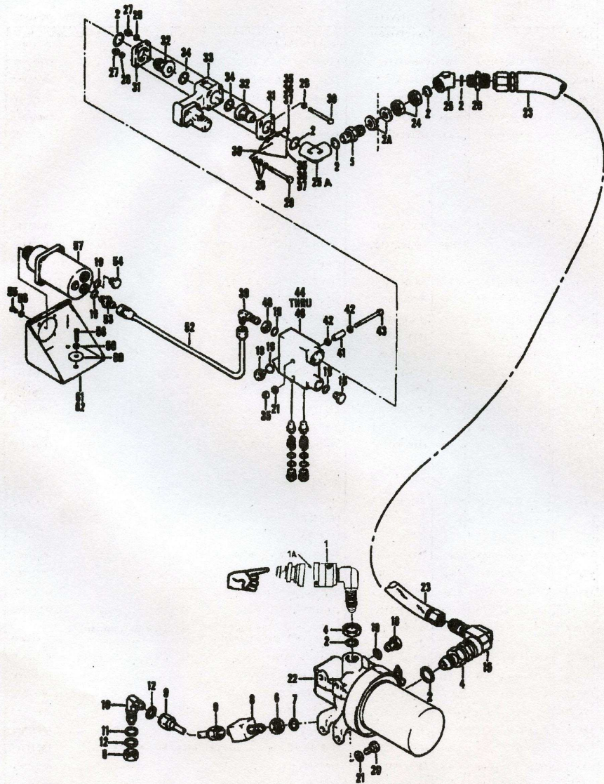
Figure 320. Fuel System Installation, Upper Section
