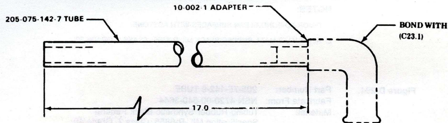
Figure D-292. Part Number: 205-075-135-19 TUBE Fabricate from: NSN 4720-00-540-3644 Material: Rubber Black Synthetic Federal Specification MIL-R-6855
