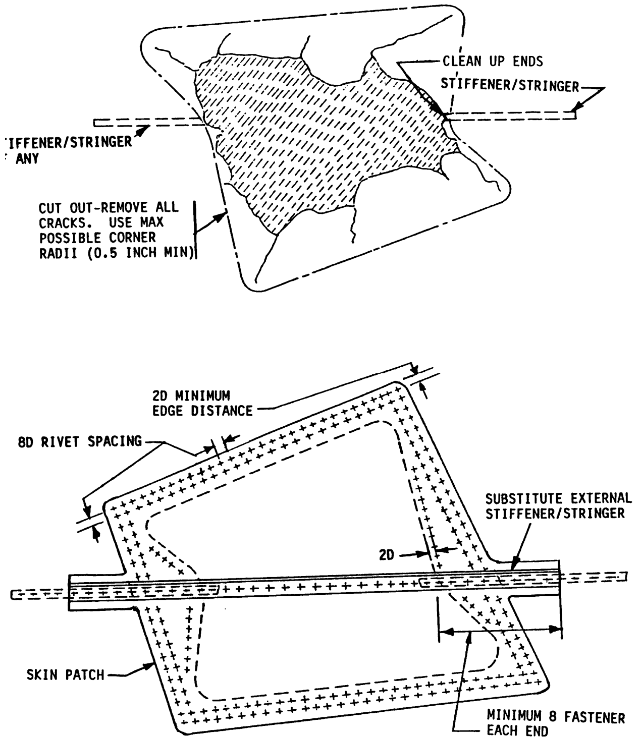
Figure 3-2. Patch Plate
