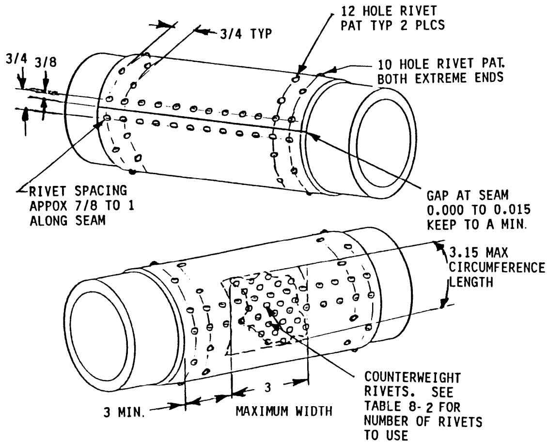
Figure 8-8. Repaired Shaft
