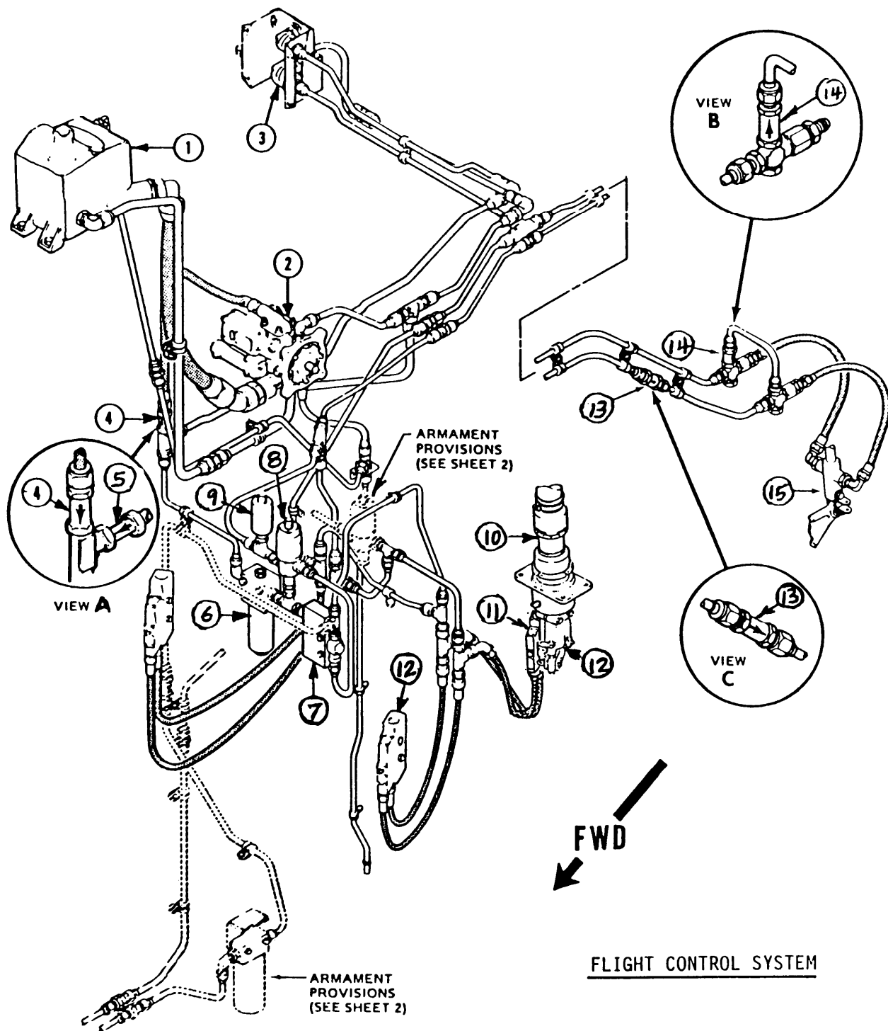
Figure 9-1. Hydraulic System (Sheet 1 of 2)
