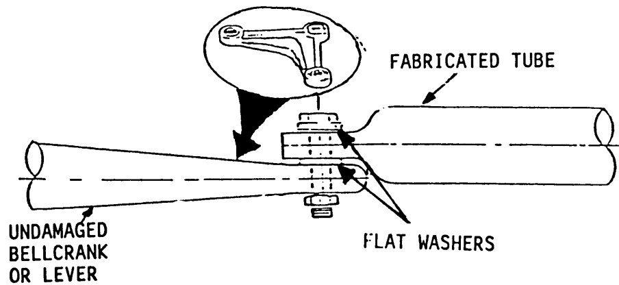
E. INSTALLATION OF FABRICATED CONNECTING LINK ON A BELLCRANK OR LEVER WITH A BEARING TYPE END
