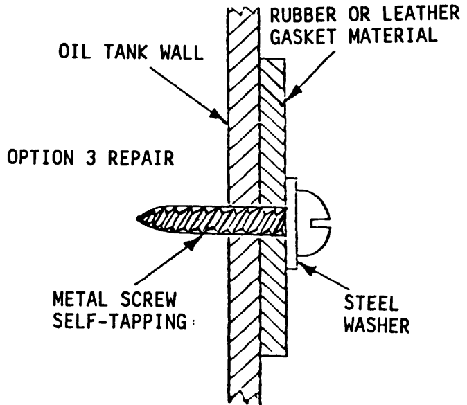
Figure 6-2. Screw, Washer and Gasket
