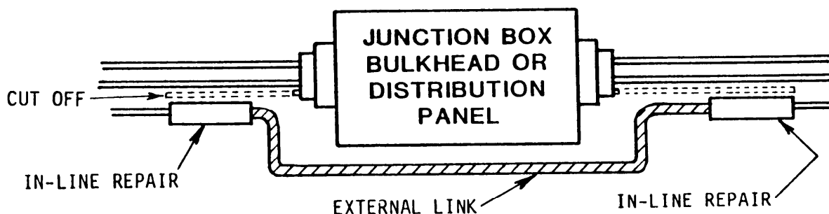
Figure 11-13. Component Bypass
