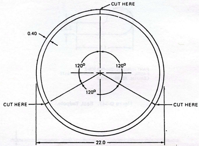
Figure D-345. Gasket
