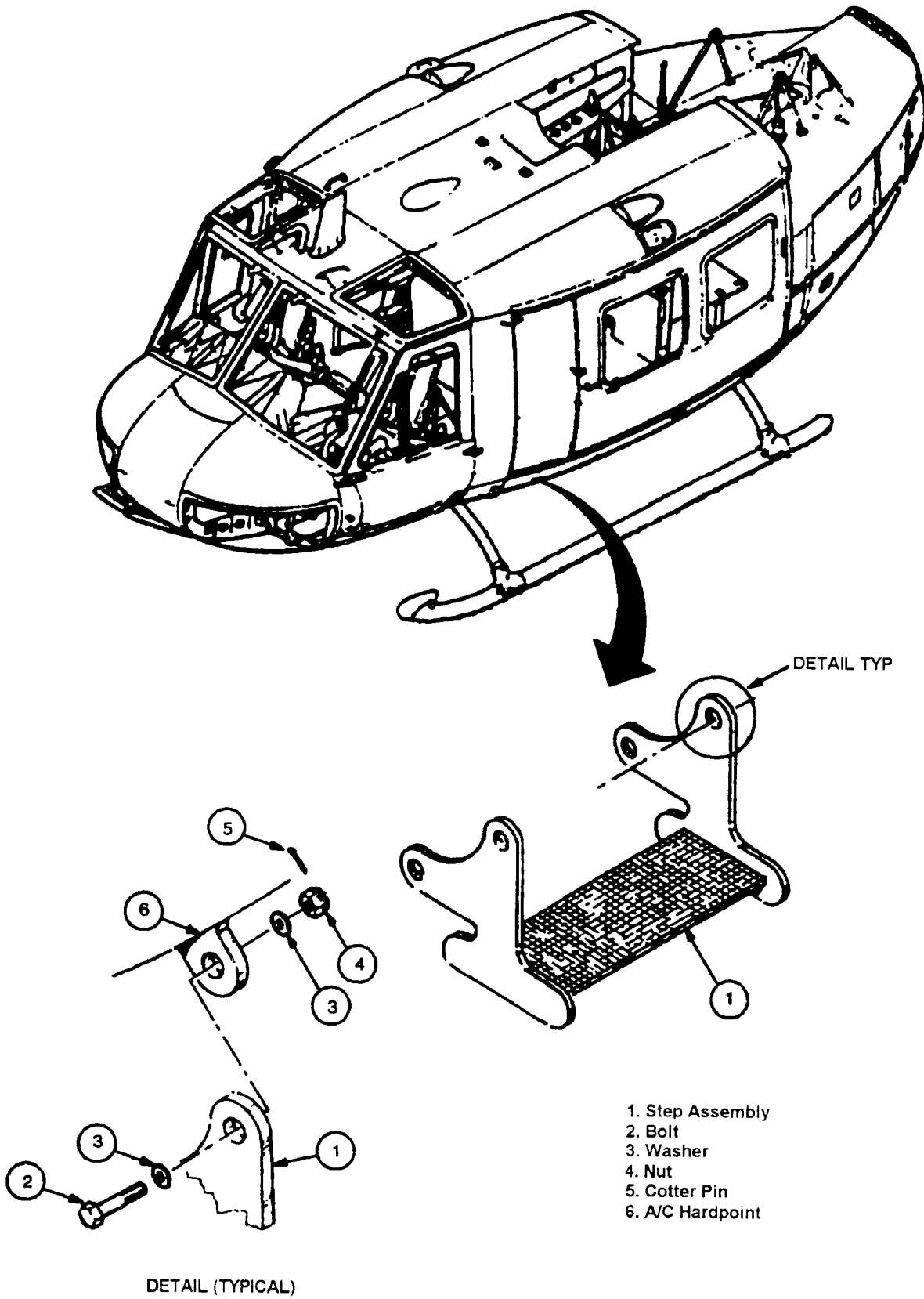
Figure 437C. Passenger Steps
