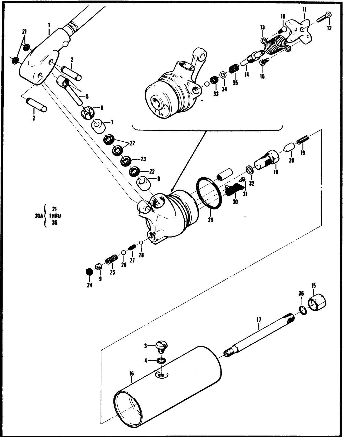
Figure G 8 Ground Support - Hydraulic Jack Pump
