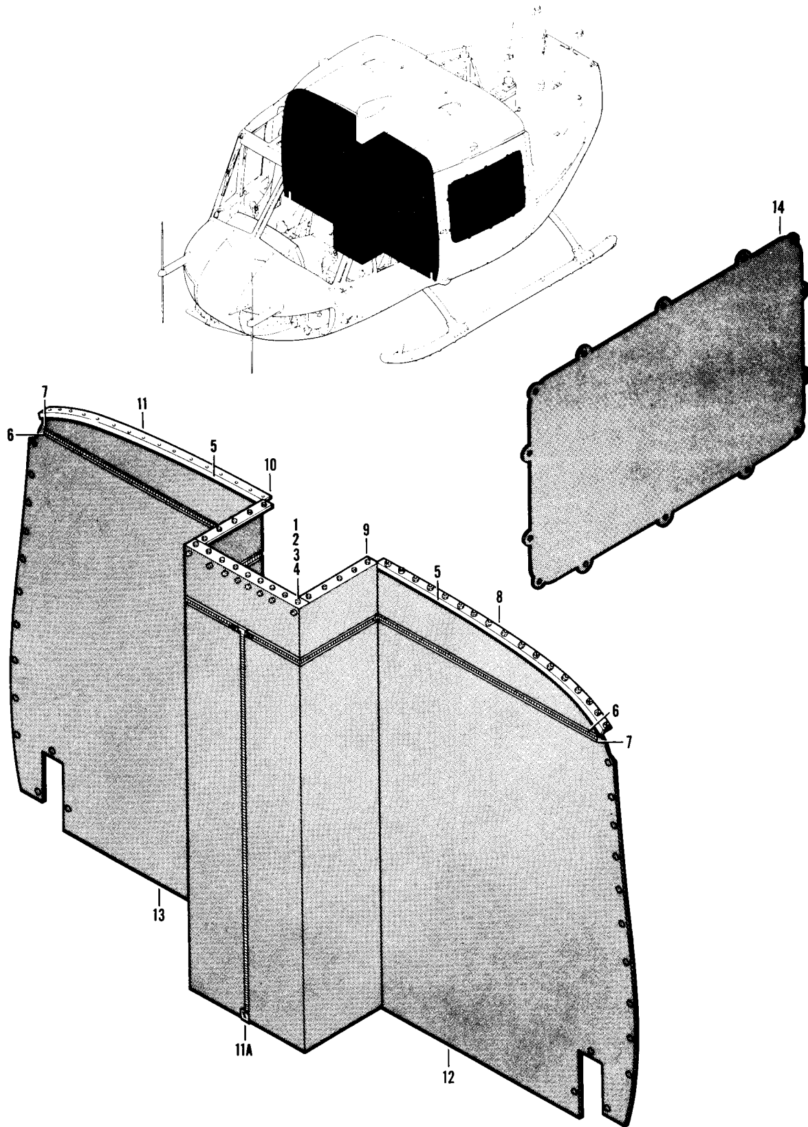
Figure 425. Curtain Installation, Blackout
