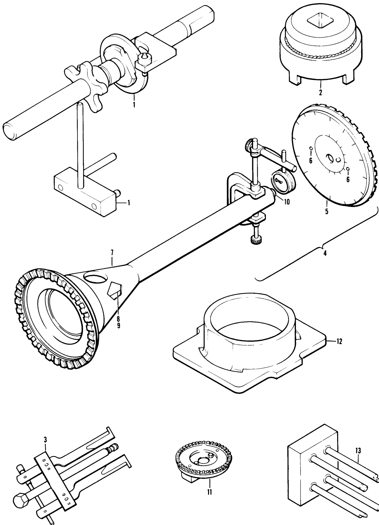
Figure A10. Airframe Tools
