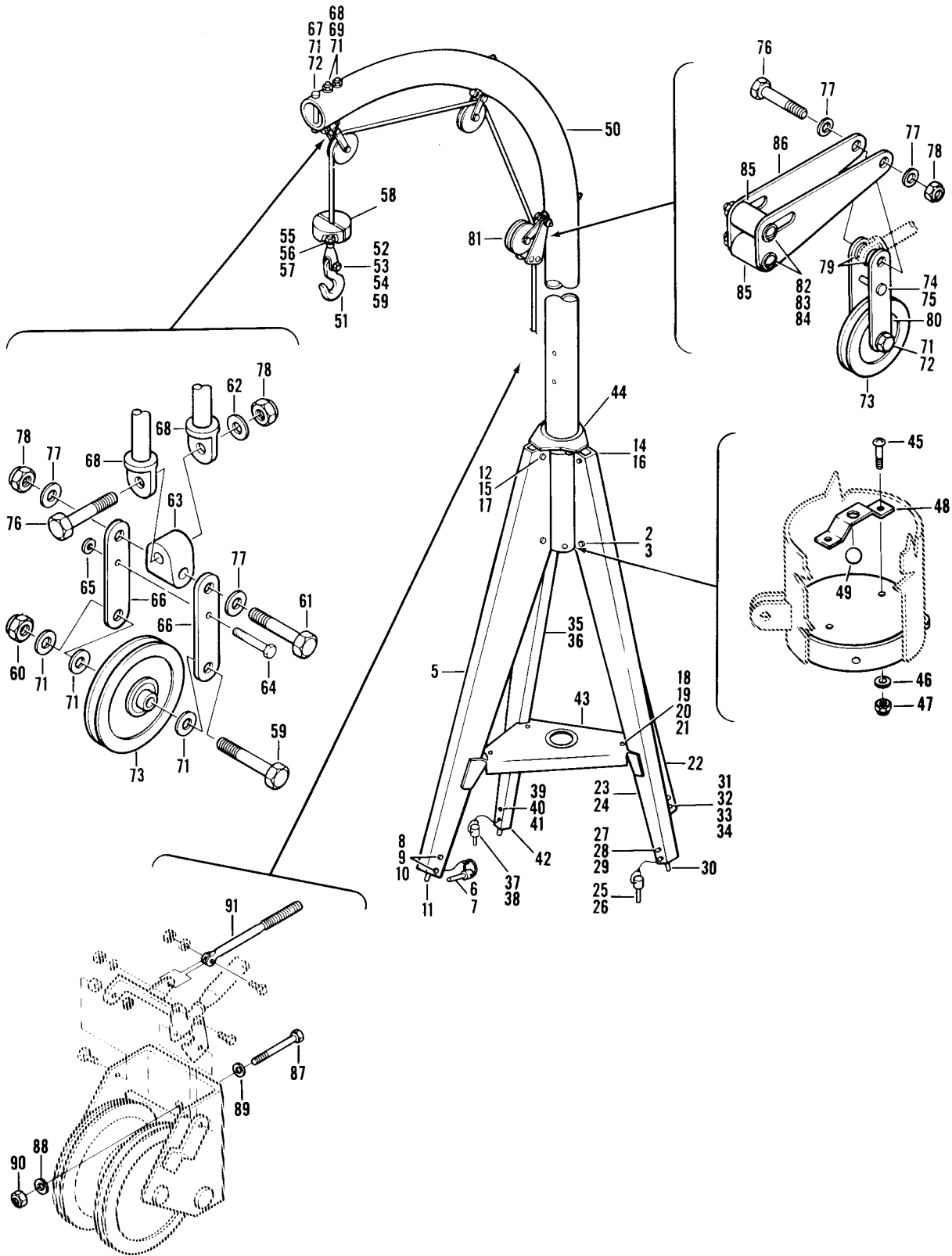
Figure G4. Ground Support Items
