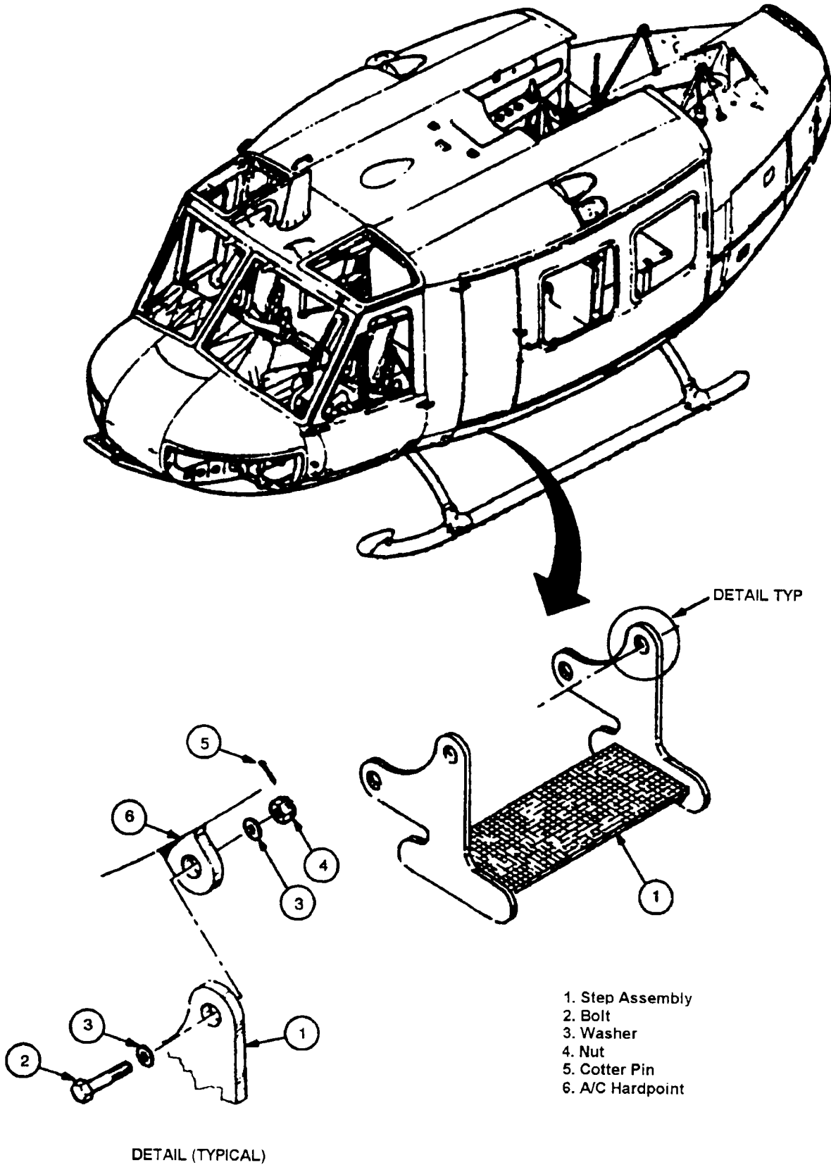
Figure 437C. Passenger Steps
