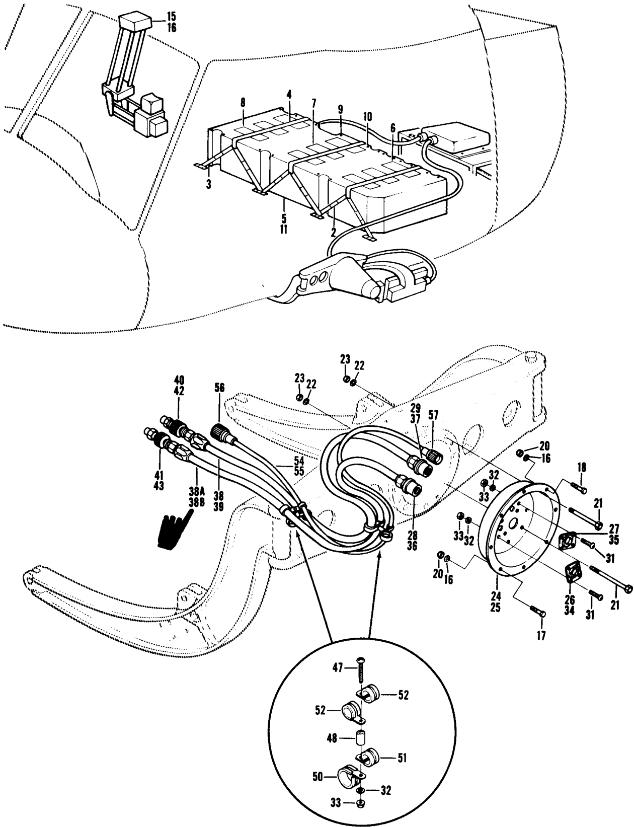
Figure 433. Armament Installation, M6
