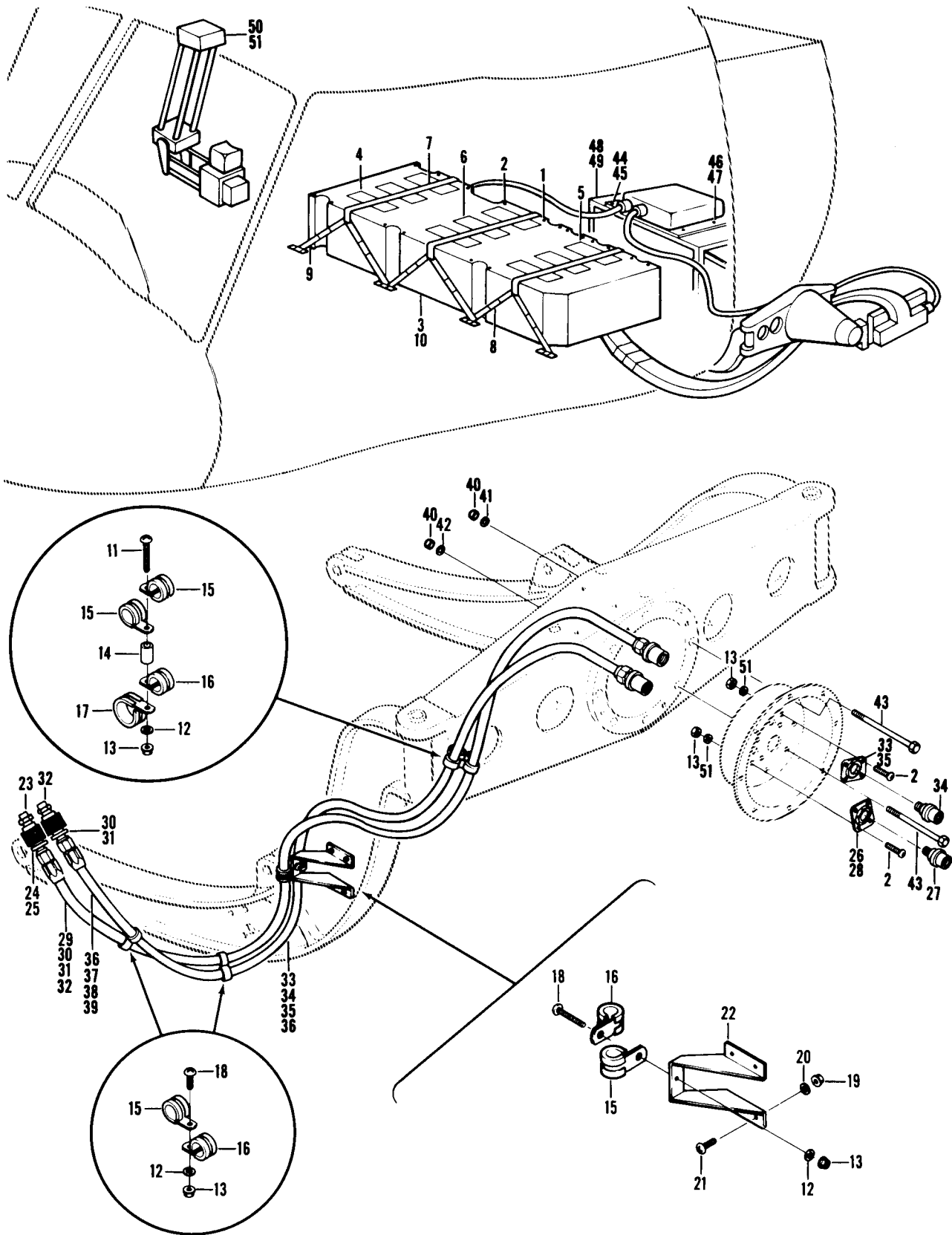
Figure 432. Armament Installation, XM6E3
