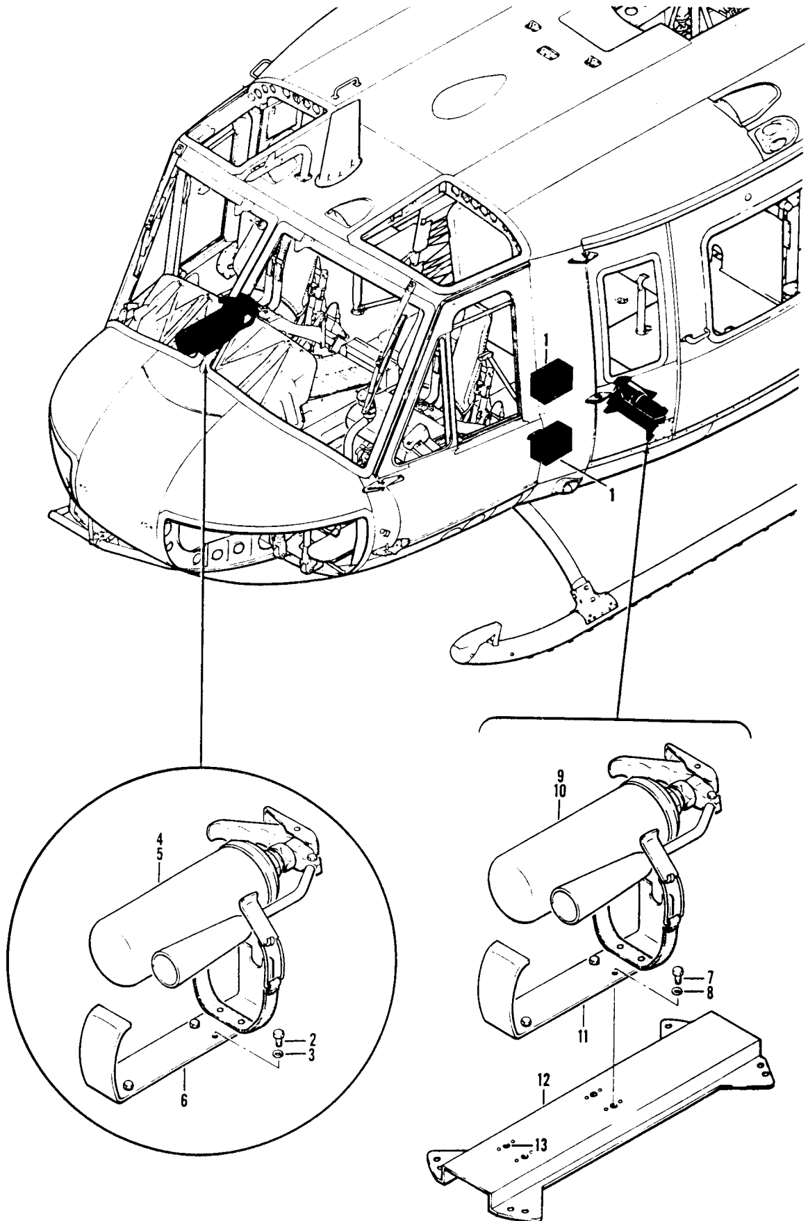
Figure 438. Fire Extinguisher and First Aid Kit Installation
