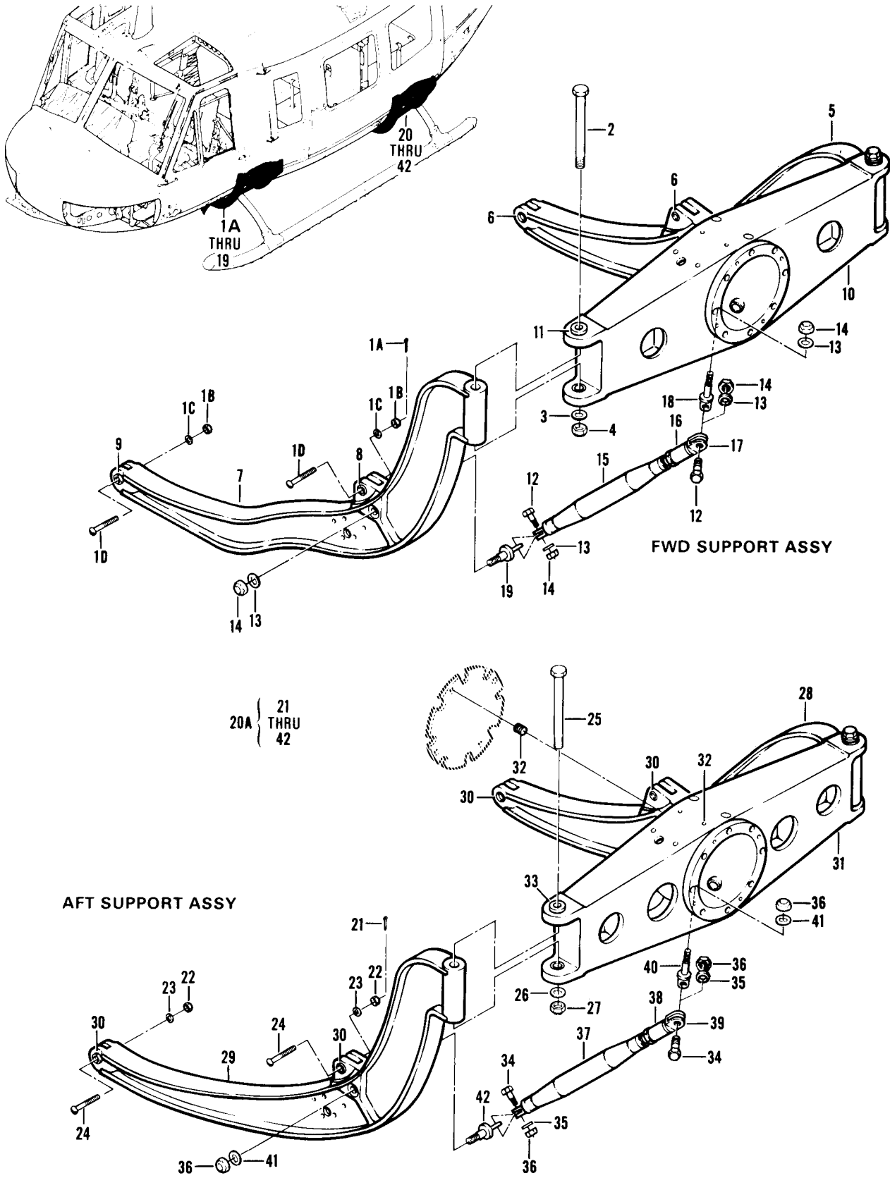
Figure 429. Installation Kit, Auxiliary Equipment
