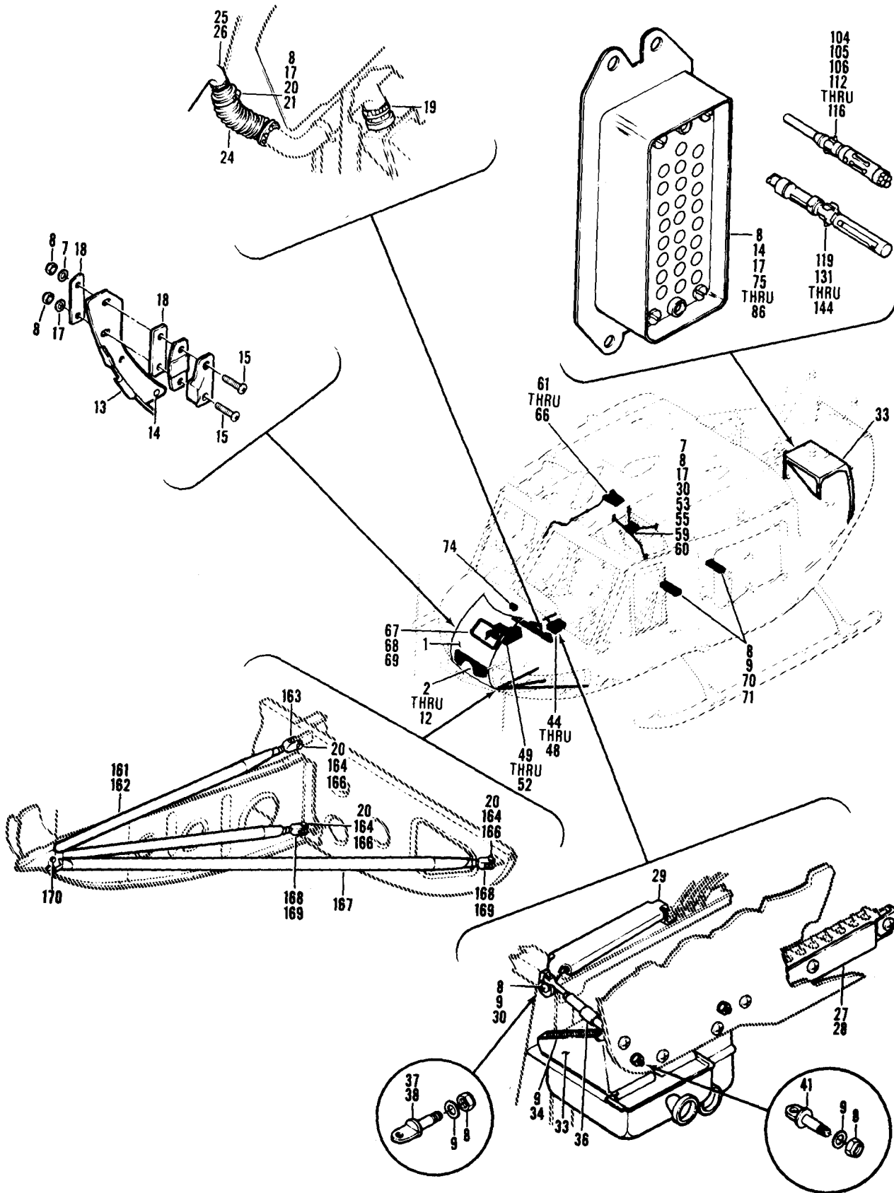
Figure 434. Armament Installation, M5 Grenade Launcher (Sheet 1 of 3)
