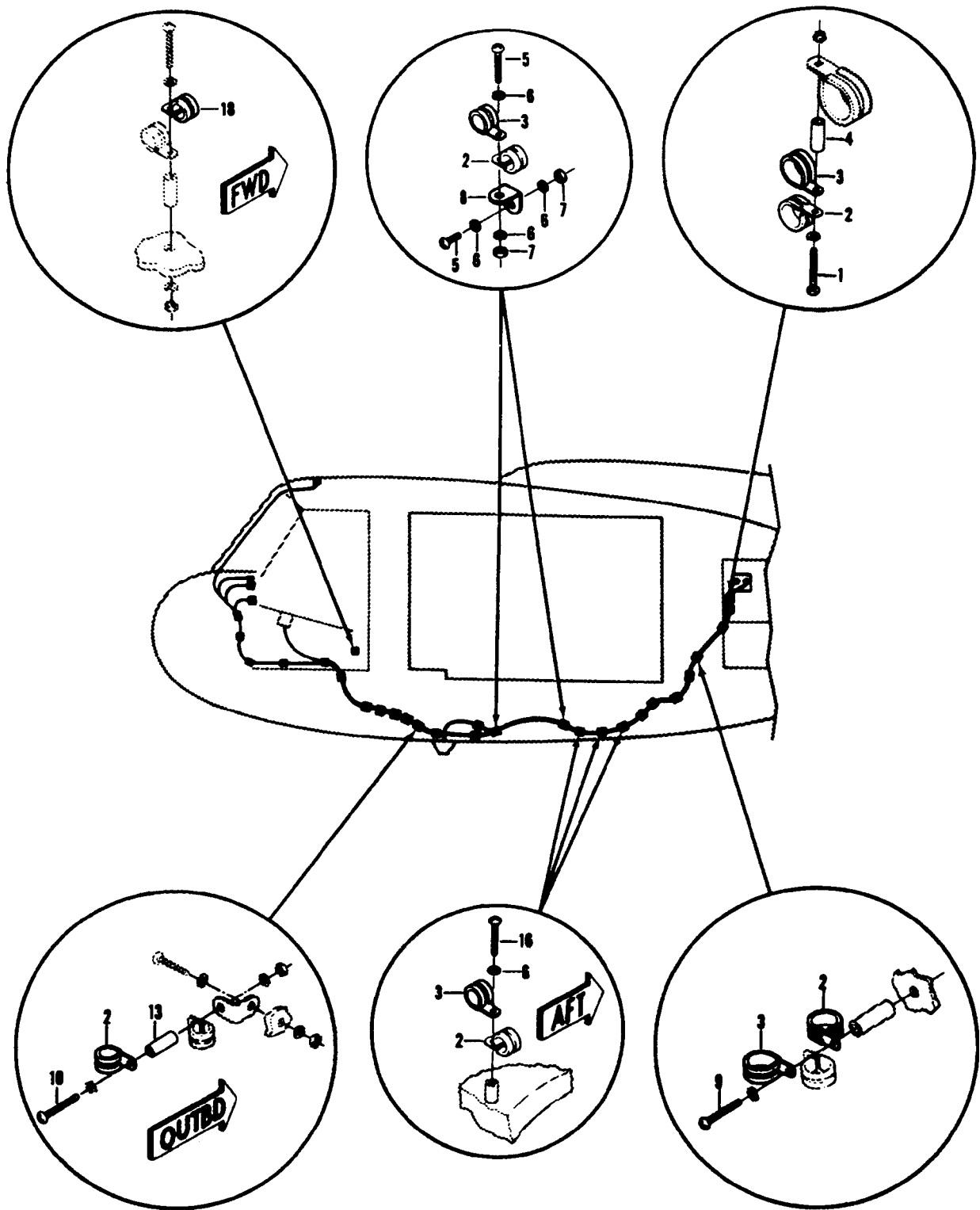
Figure 437B. Kit Installation, DME (Sheet 1 of 4)
