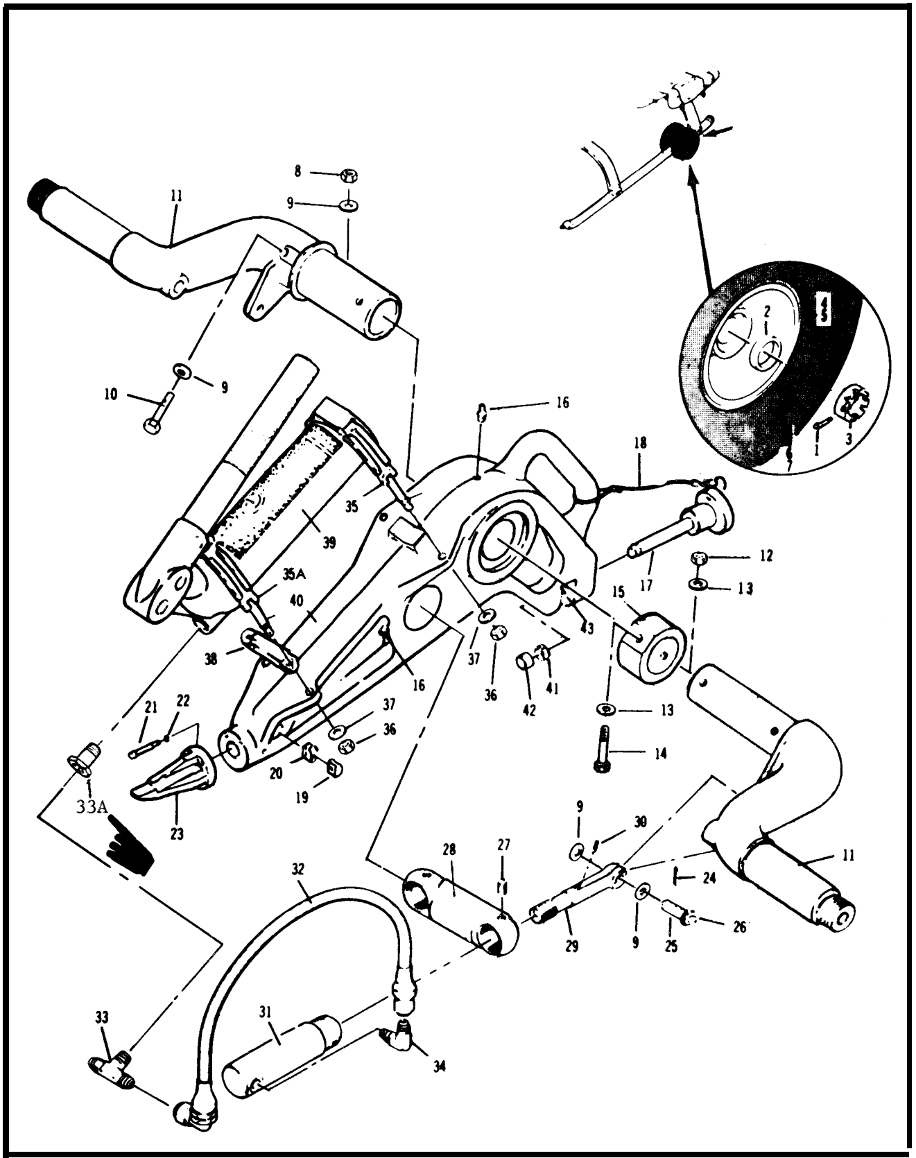
Figure G7 Ground Handling Gear Assembly (sheet 1 of 2)
