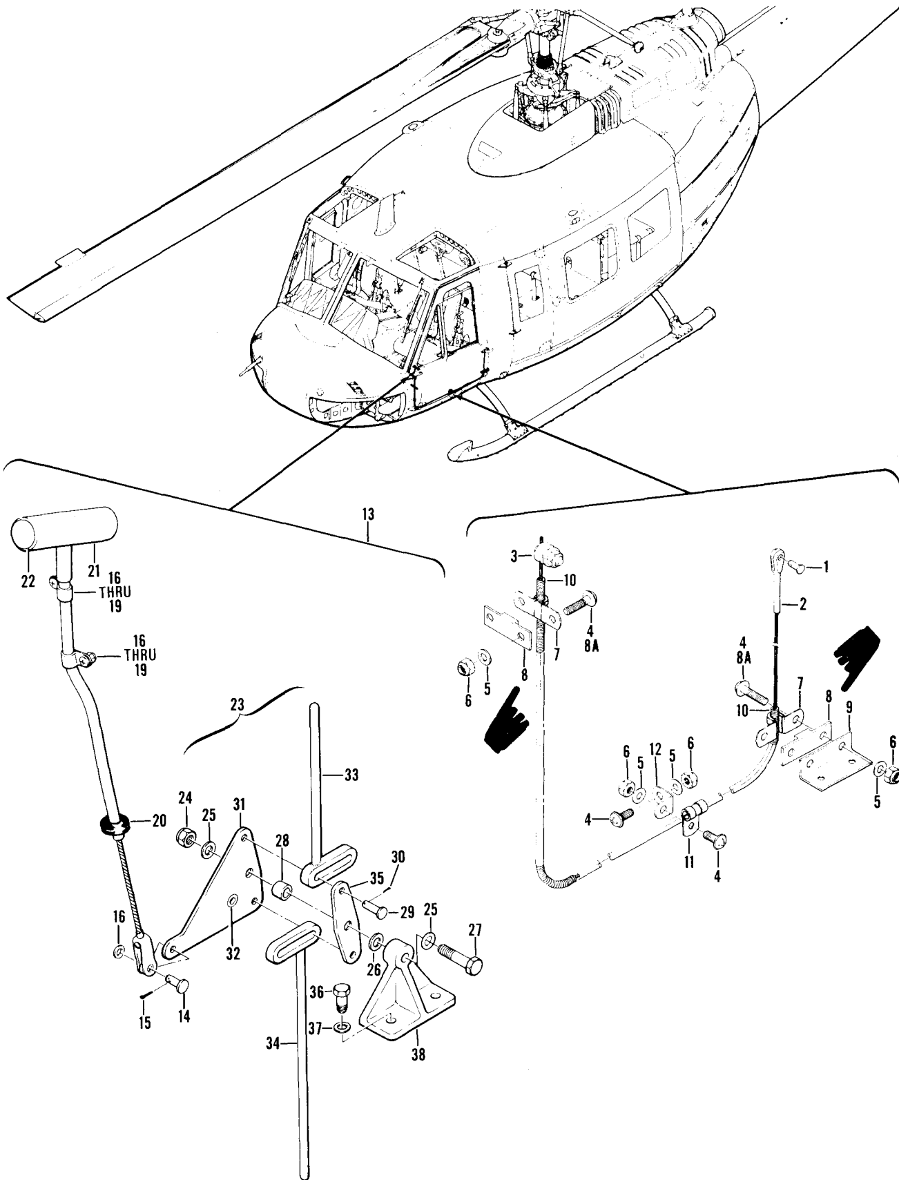
Figure 440. Cable Installation, Striker Ejection
