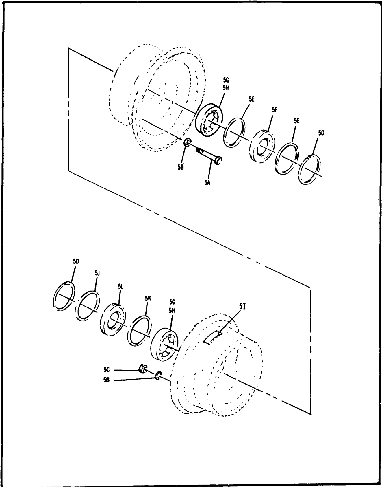
Figure G7 Ground Support — Ground Handling Gear Assembly (Sheet 2 of 2)
