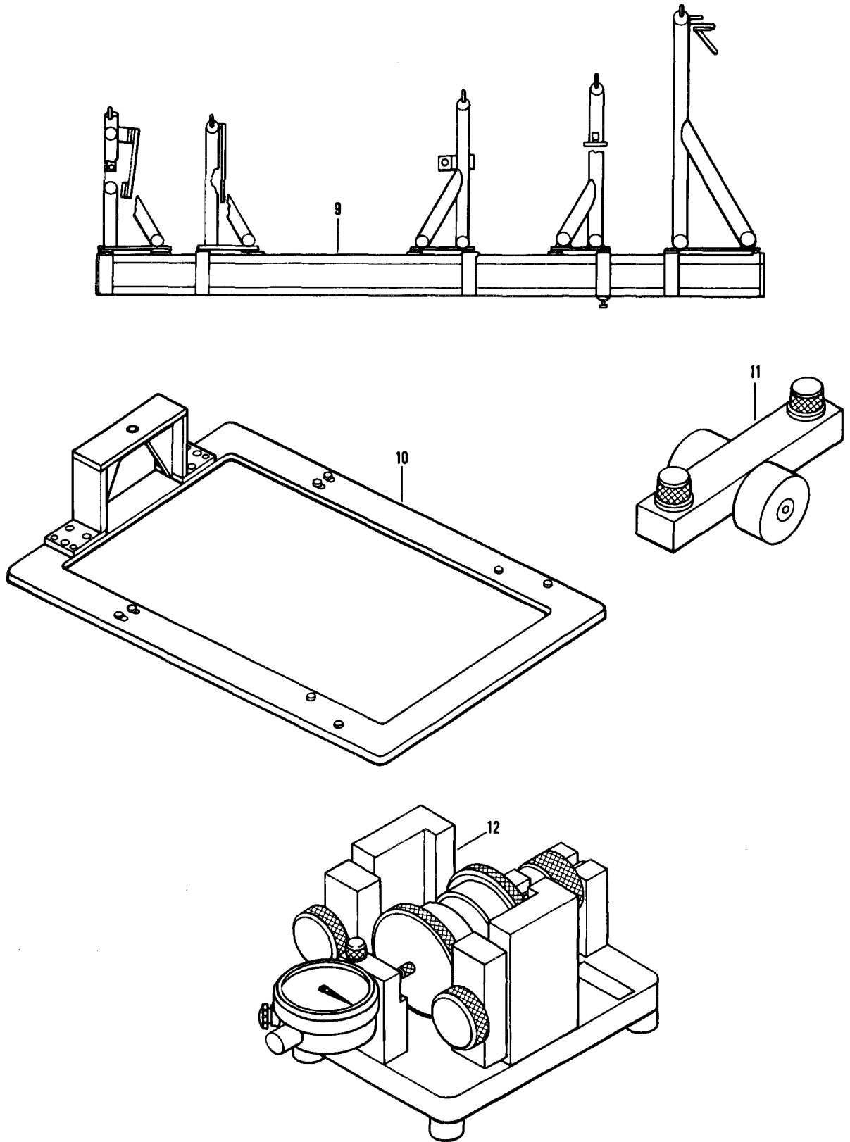
Figure A5. Airframe Tools (Sheet 2 of 2)
