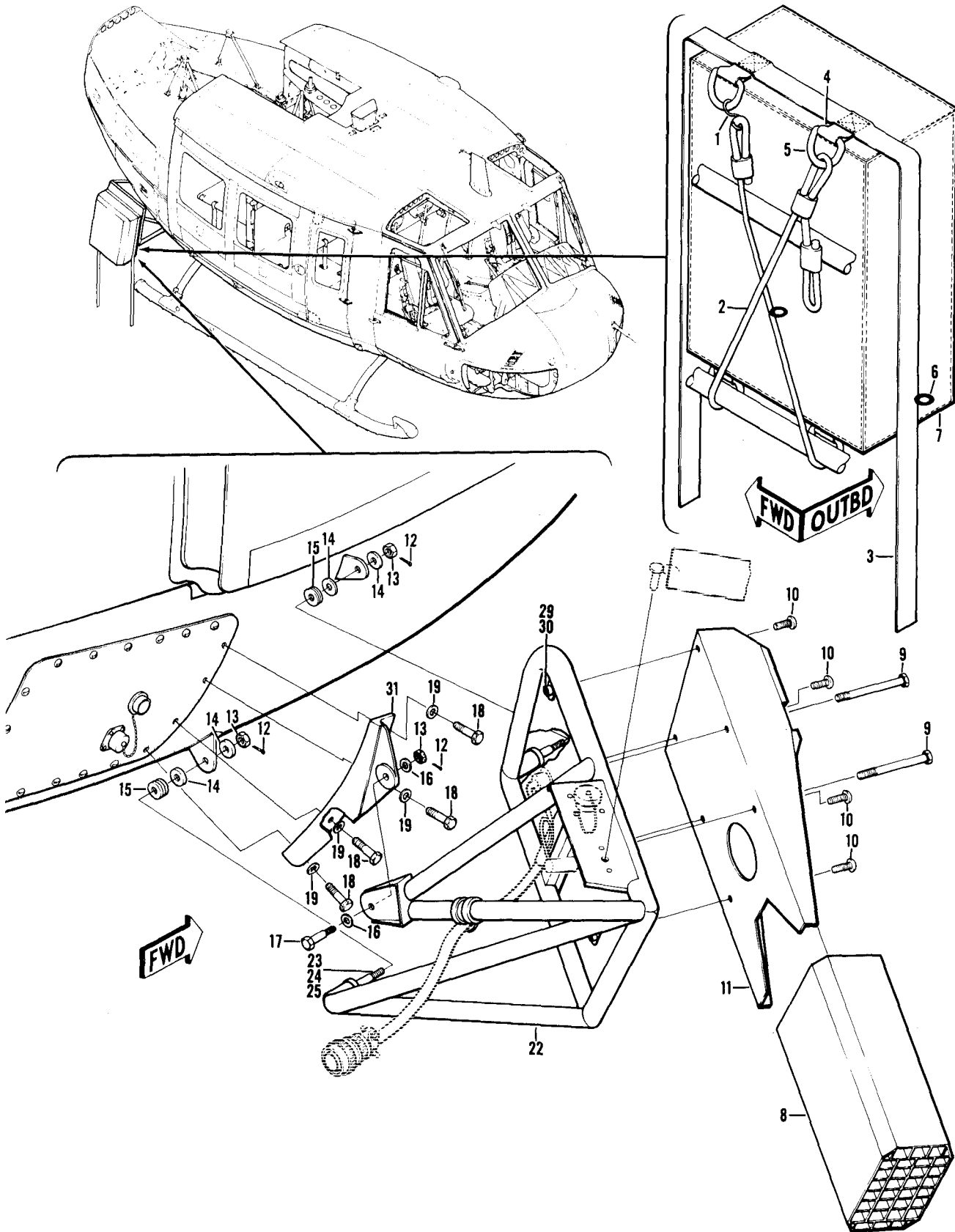
Figure 430A. Flare and Chaff Installation, M130 (Sheet 1 of 2)
