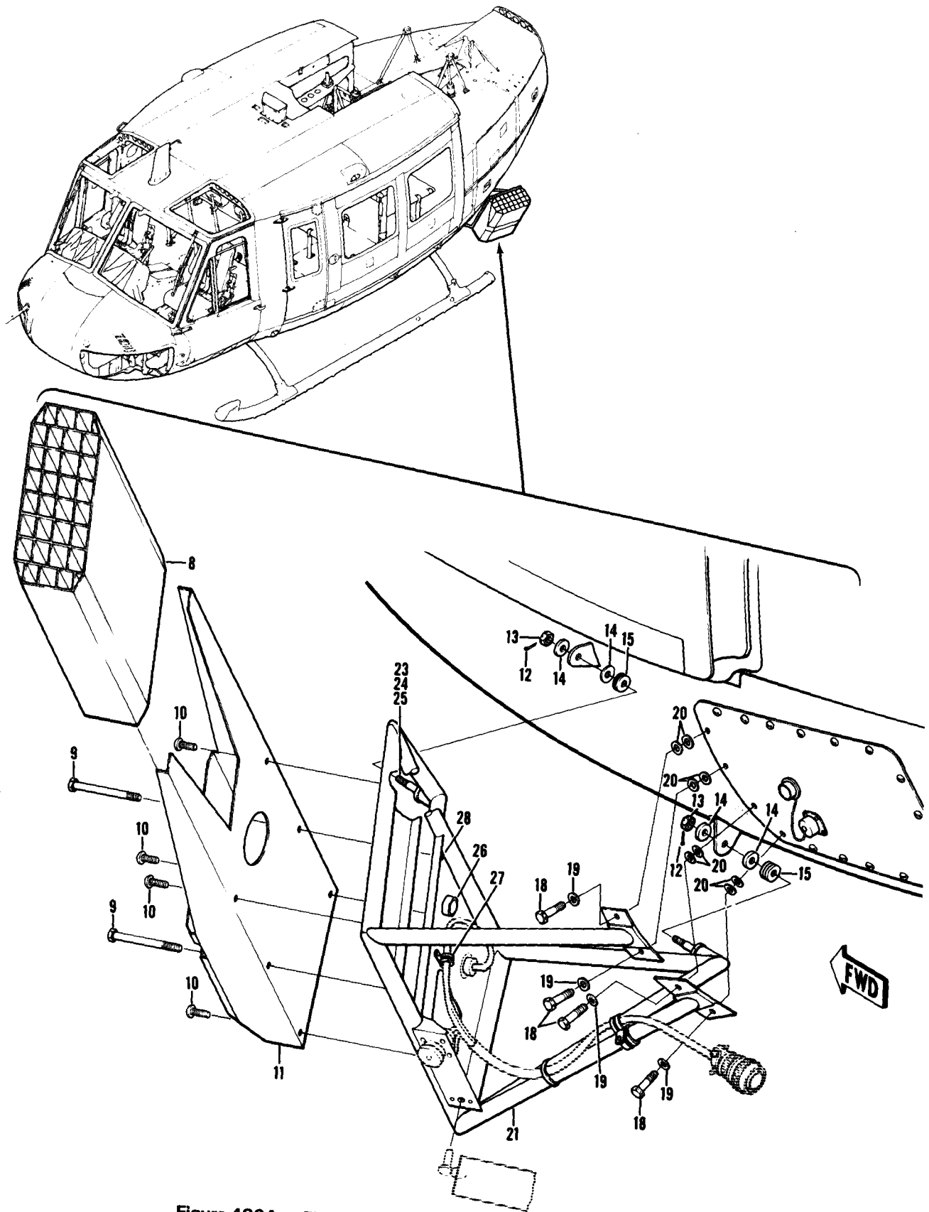
Figure 430A. Flare and Chaff Installation, M130 (Sheet 2 of 2)
