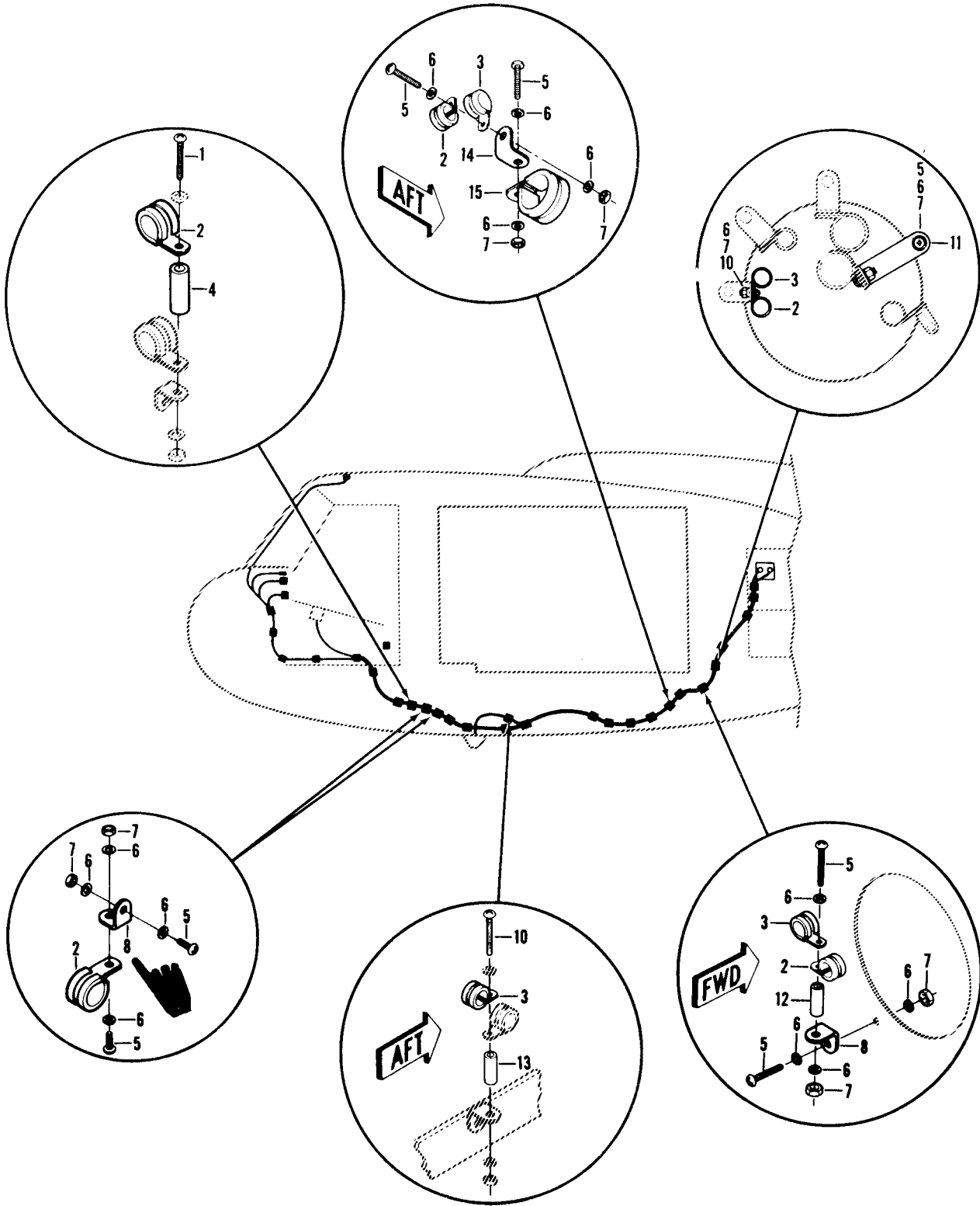
Figure 437B. Kit Installation, DME (Sheet 3 of 4)
