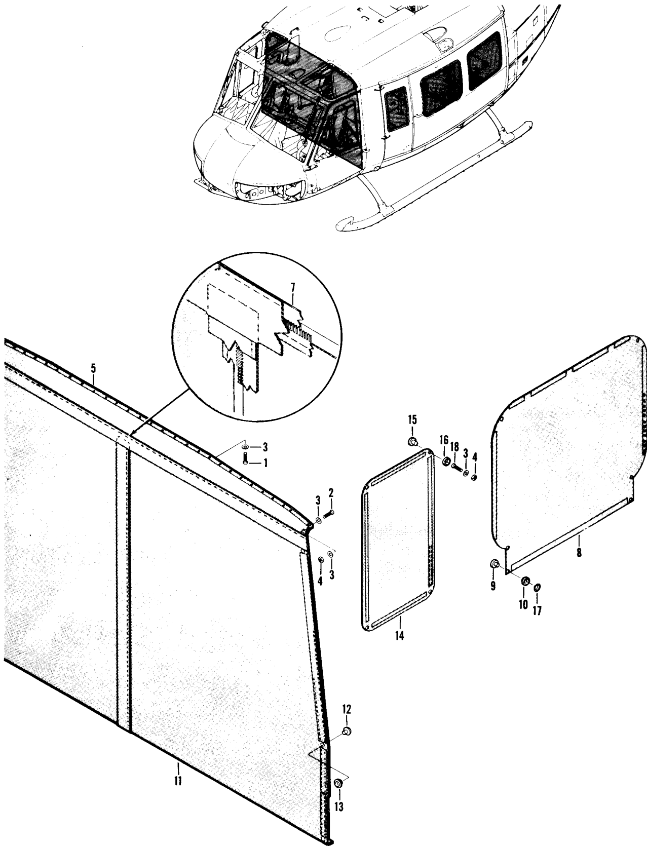
Figure 426. Curtain Installation, Blackout
