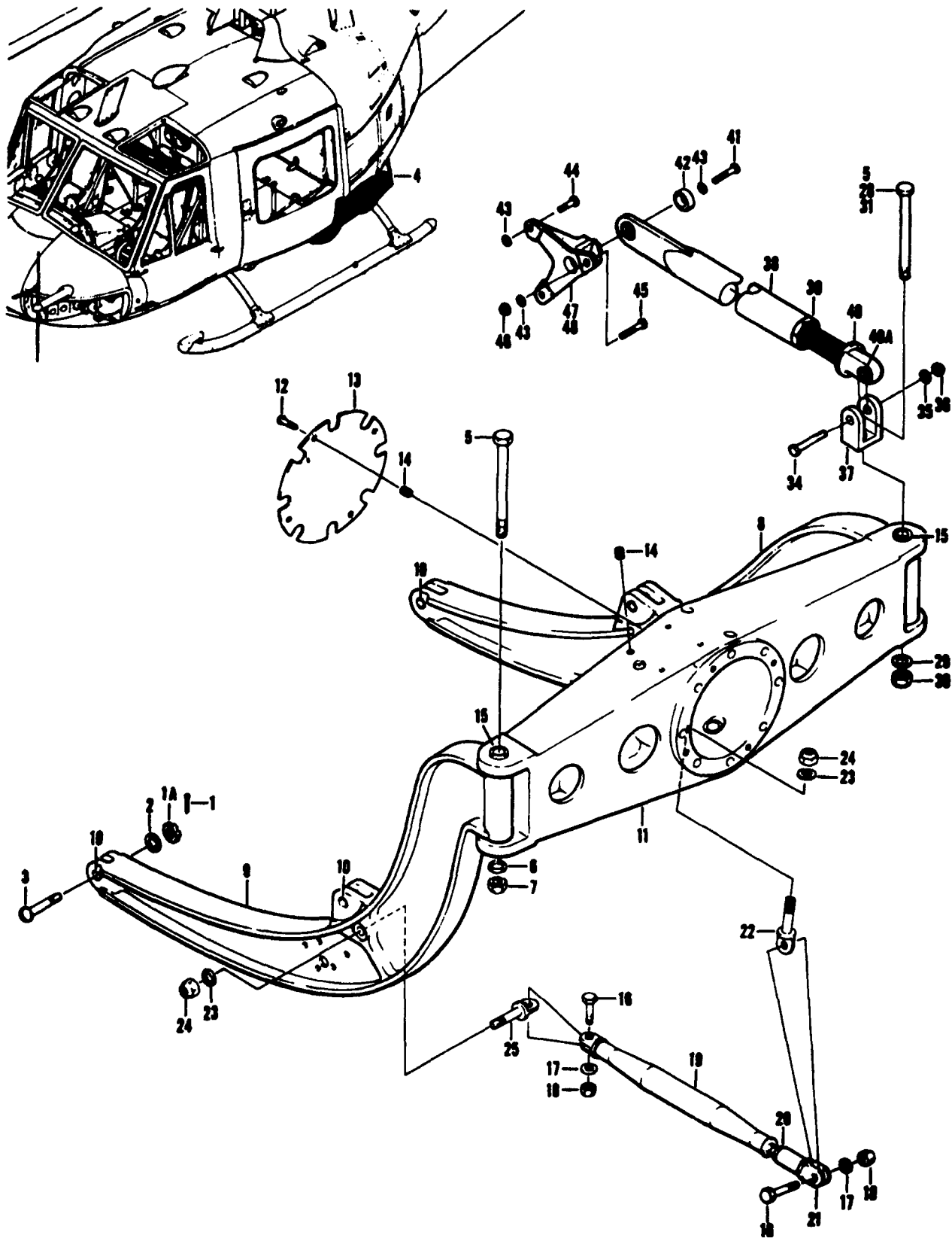
Figure 428. Support Assembly, External Stores
