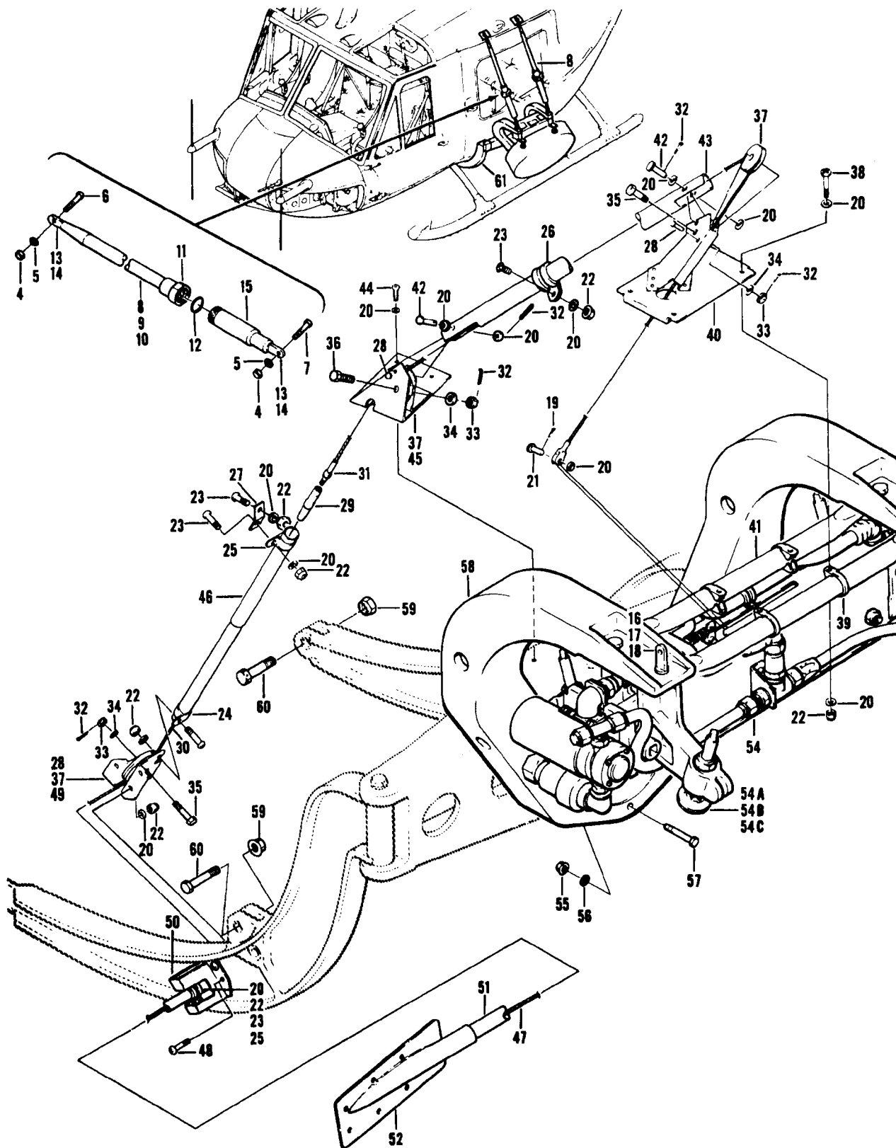
Figure 437. Armament Installation M56
