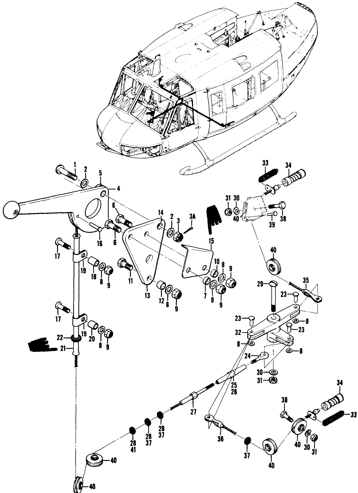
Figure 442. Control Installation, Jettison Emergency
