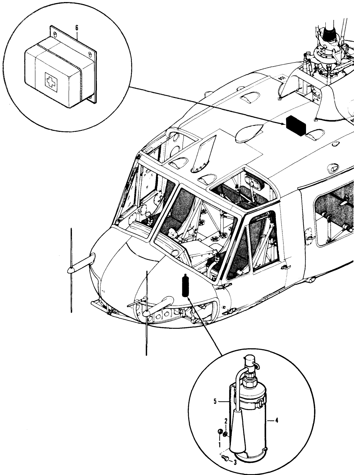
Figure 439. Loose Equipment Installation
