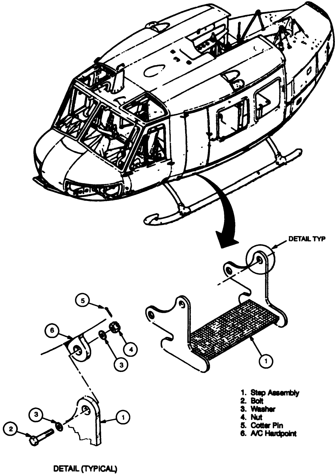
Figure 437C. Passenger Steps.
