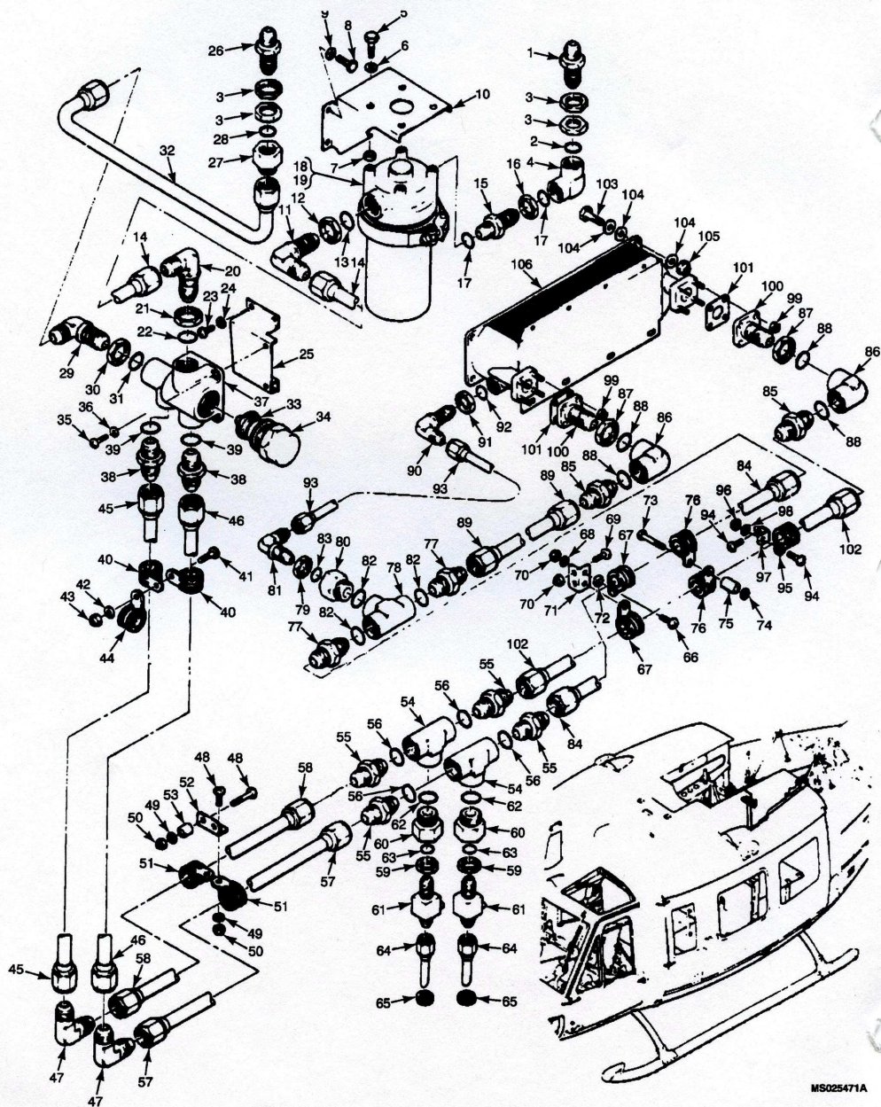
Figure 175. Transmission Oil Cooler Installation
